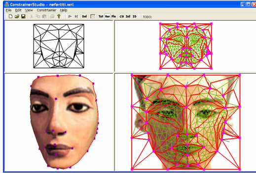
Figure 7: Matchmaker GUI.
